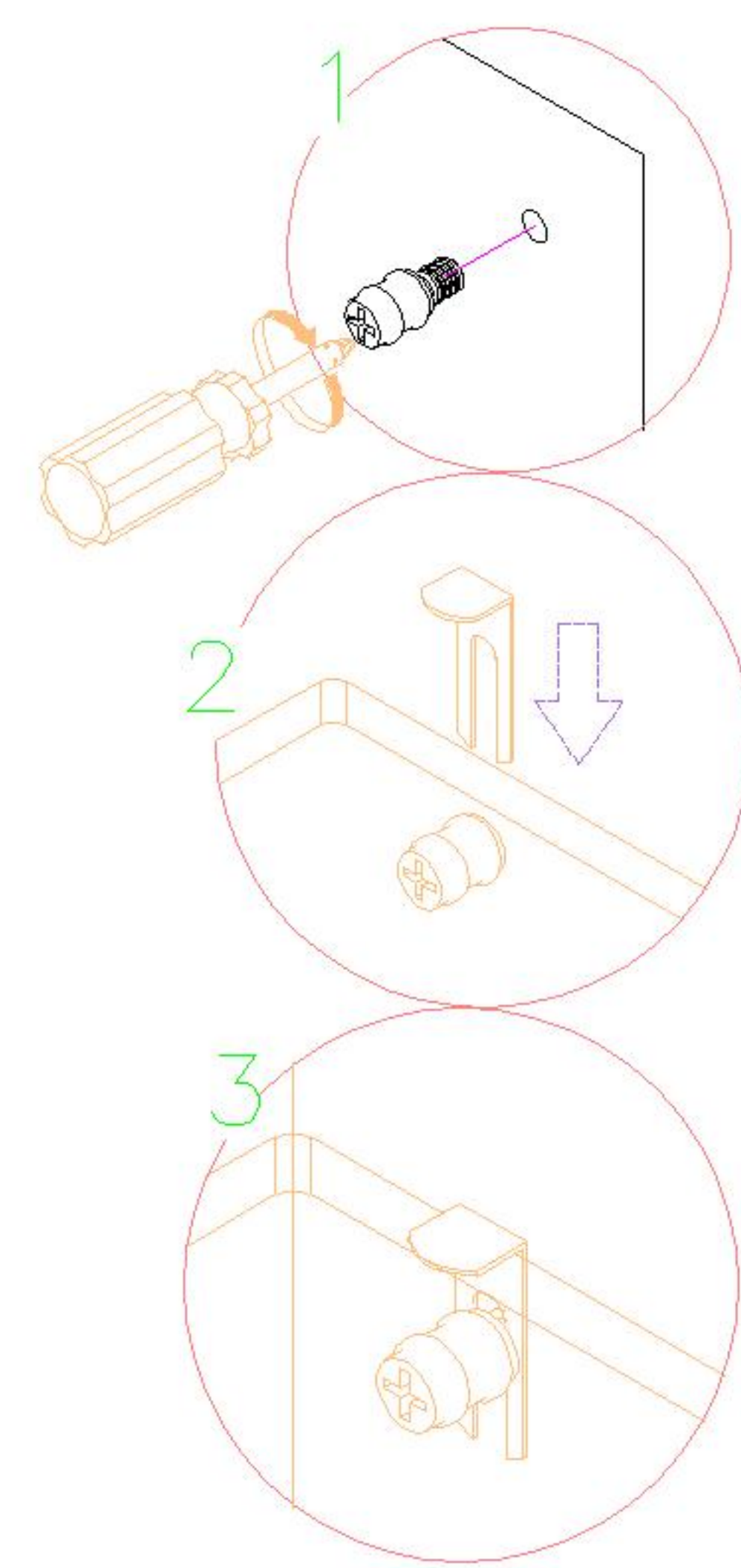
玻璃层板托杆/叉 Glass laminate bracket/fork
